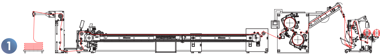
Compacting line with 9 m tenter frame, 2-roller B-Kompact 600 open width felt compactor, non stop winder.
