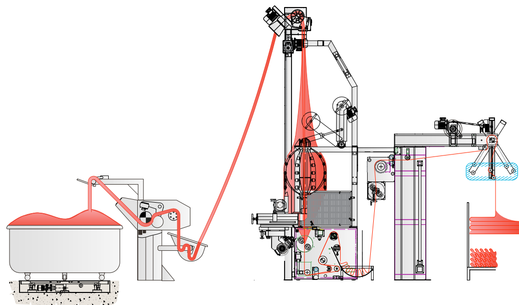
Rope opener & slitting line tension less with relax scray
