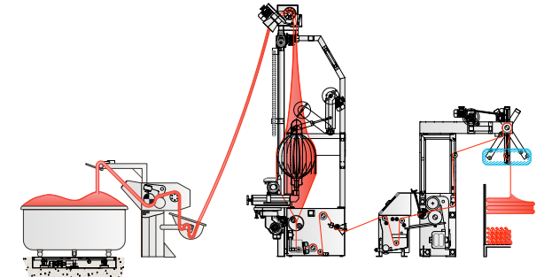
Rope opener & slitting line with squeezing padder and TNK washing tank
