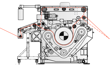
In-line B-Shrink open width rubber belt compactor
