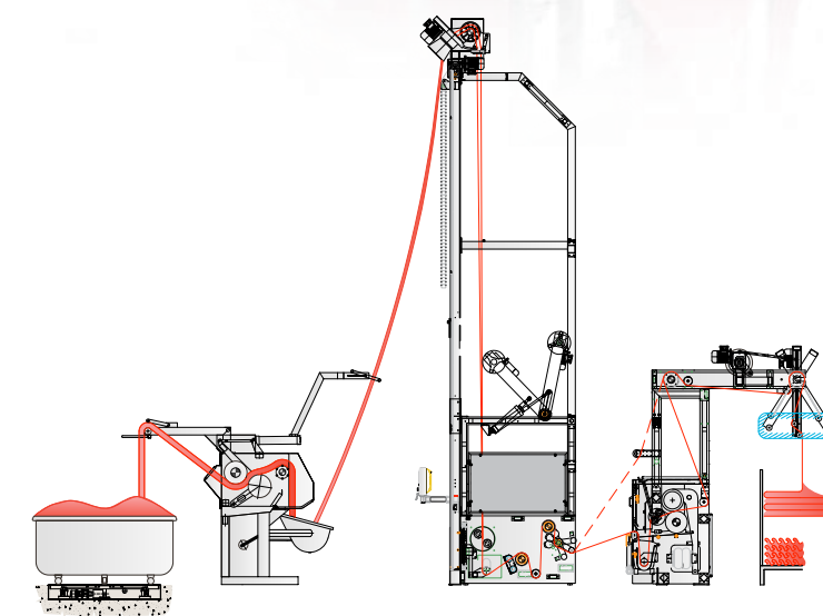
Rope opener line with squeezing padder
