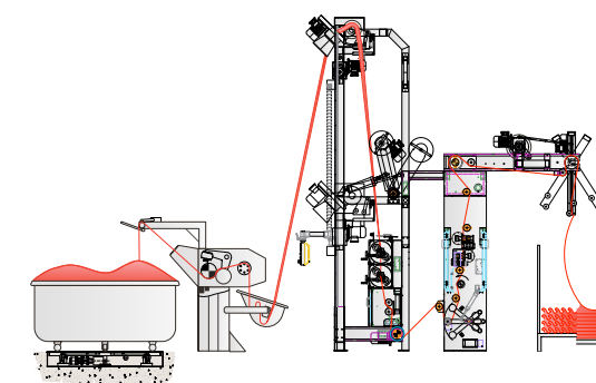
Rope opener line with hydro-extractor
