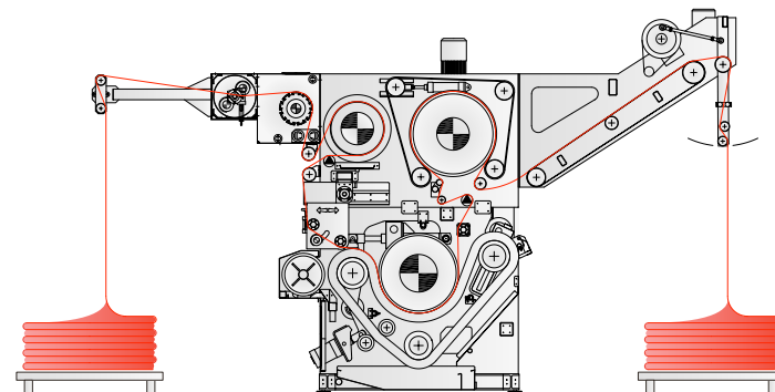
B-Shrink open width rubber belt compactor Stand Alone
