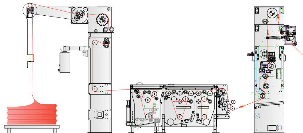
Happy Scour EVO PLUS with hydro-extractor
