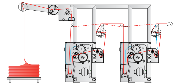
Open width squeezing padder with load cells
