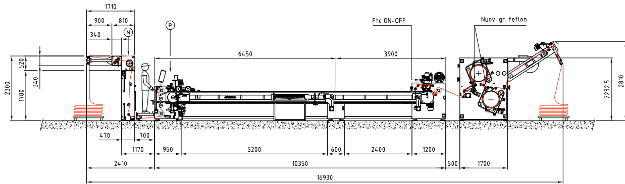
Bianco® B-Kompact Compactor with Tenter Frame and Selvedge Gluer, Dryer and Cutter
