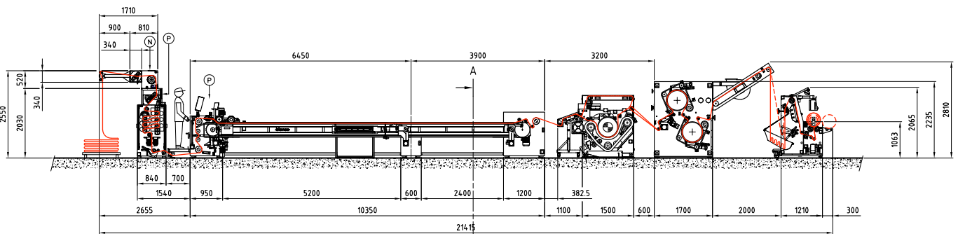
Bianco® B-Kompact and B-Shrink Compactors with Tenter Frame, Weltstraightener and non stop Winder
